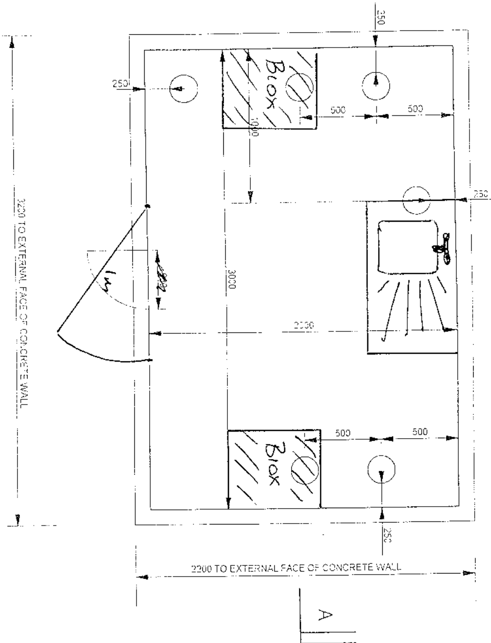
OVERALL PLAN OF KIOSK AREA (SCALE 1:25)
